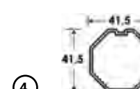
④ Int. Tube Drive Shaft profile
