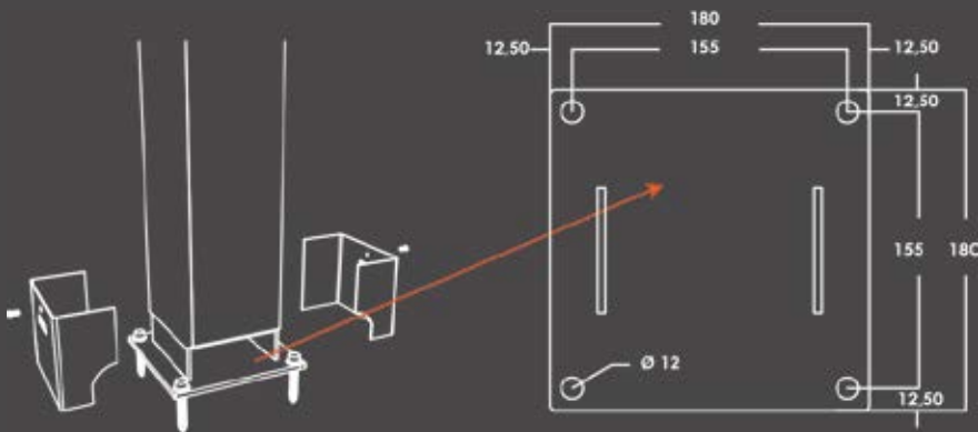
■ Column support base 130 x 130
