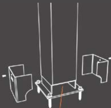
Column support base 130 x 130
