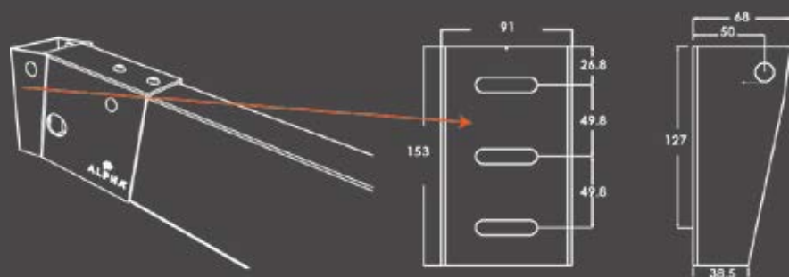
■ Wall - ceiling support Base 130 x 65cm
