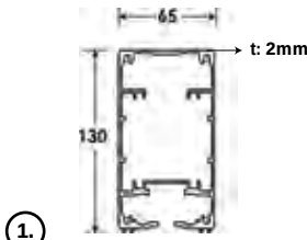
① Side Guides
