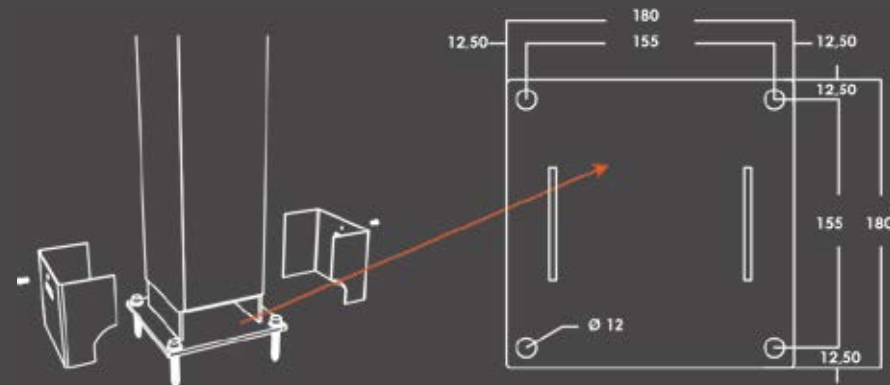
■ Column support base 130 x 130
