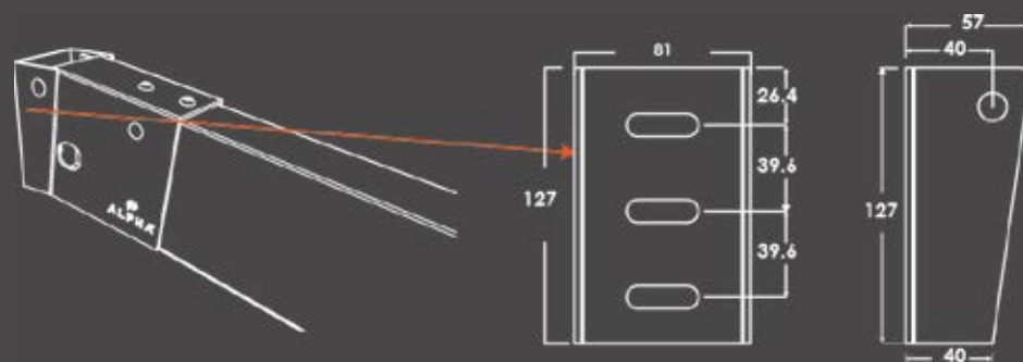
Wall - ceiling support Base
